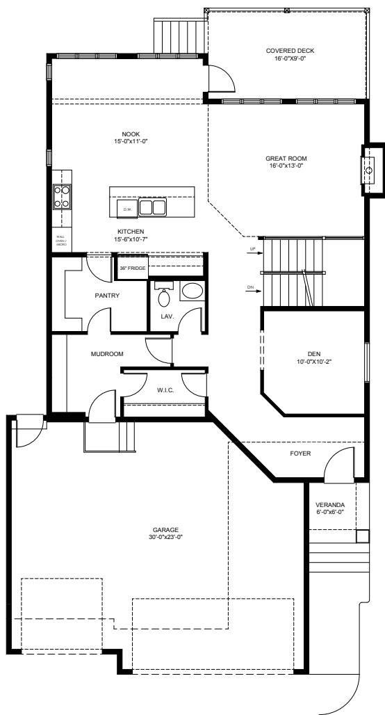
MAIN FLOOR 1181 sqft
