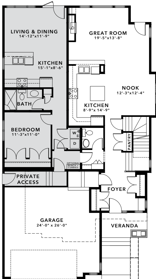
MAIN FLOOR
